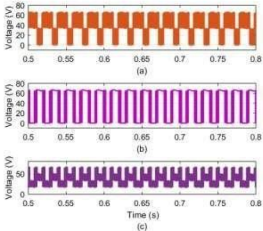
Fig.7. (a) V_{AV} (b) V_{BN} (c) Common mode
