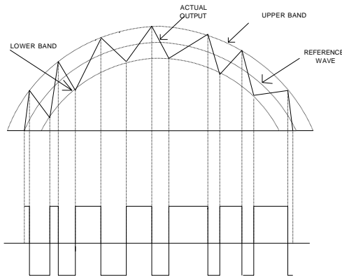
Fig. 1. The model waveform of Hysteresis control
