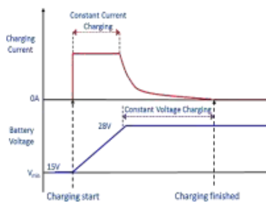
Fig 1. Stages in CC-CV charging method
