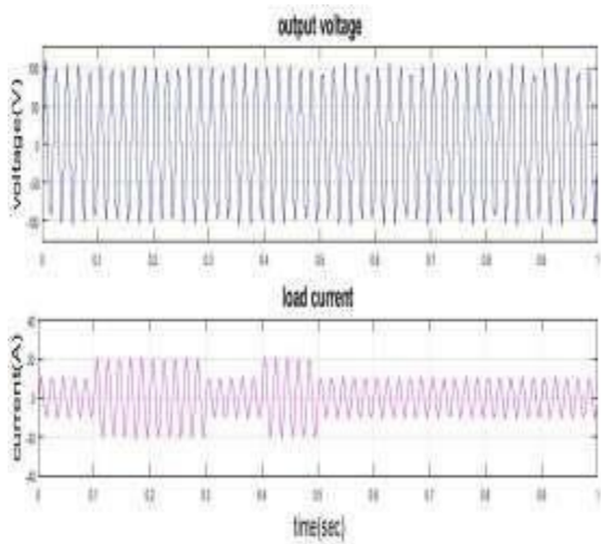
Fig.10 Waveform of the output voltage and current
