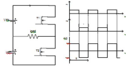
Fig. 2. Schematic of HBI
