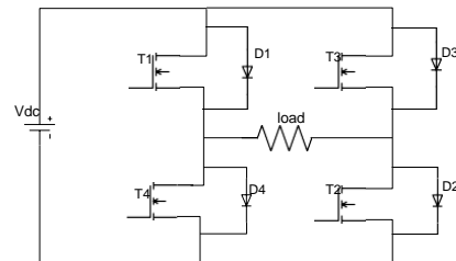
Fig. 3. Schematic of Single phase FBI
