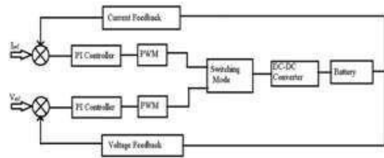
Fig 3. Control Loop Block Diagram for the CC-CV Charging Scheme
